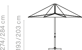
Inumbra medium + concrete base 71/81
