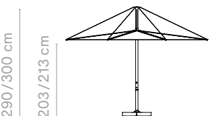
Inumbra large + concrete base 71/81
