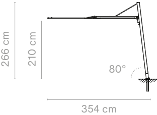
Carré simple tilted + floor fastening spacer plate
