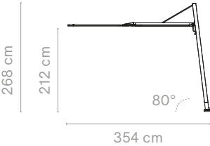
Carré simple tilted + floor fastening spacer plate
