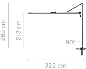
Sensu single square straight + floor fastening spacer plate & pole extension
